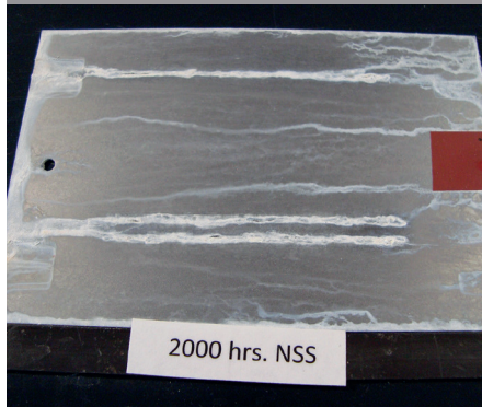
Scratch test 2 mm Protalloy®
